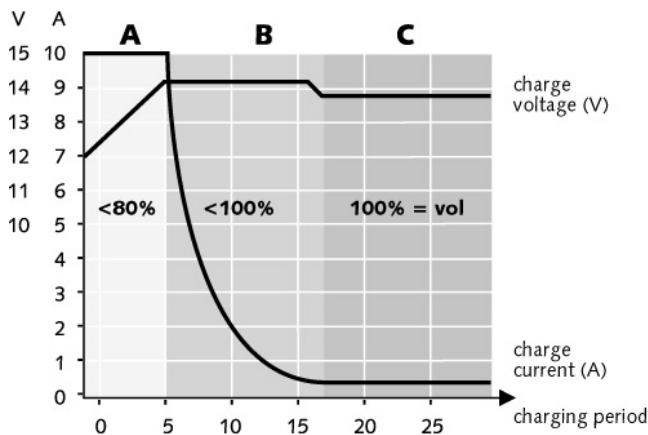
Figure 1: Charge characteristic
